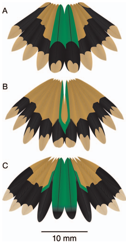
FIG. 3. Tail patterns of (A) adult female Chaetocercus berlepschi (Emeraldas Woodstar), (B) adult female C. bombus (Little Woodstar), and (C) juvenile male C. berlepschi .
