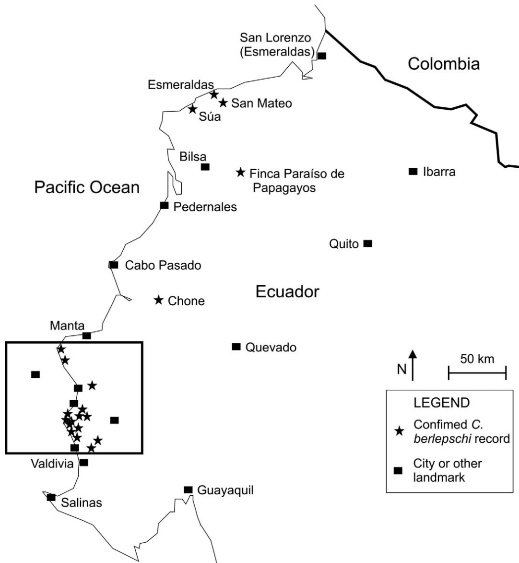
FIG. 1. Western Ecuador showing confirmed records of Chaetocercus berlepschi (Esmeraldas Woodstar) as well as larger cities and landmarks.
