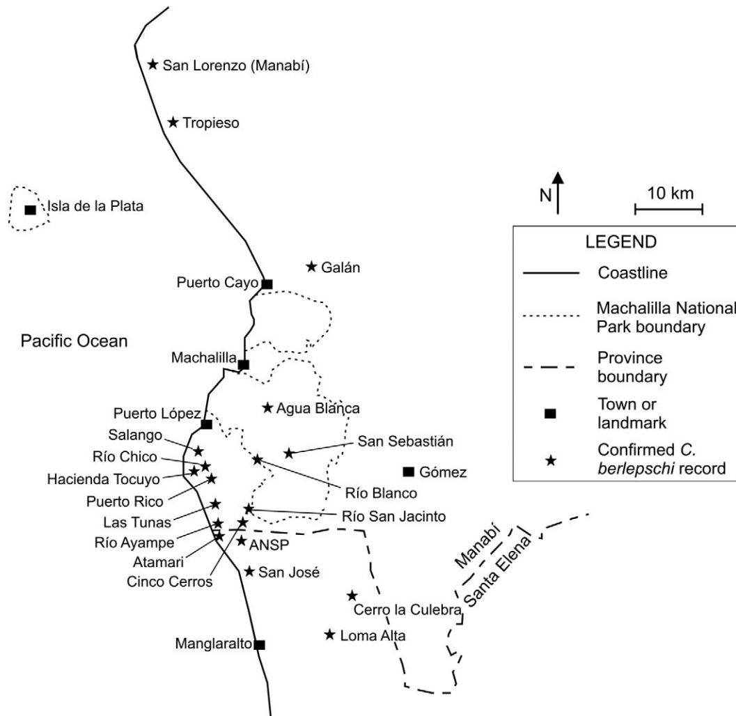
FIG. 2. Focal area of study (inset in Fig. 1) showing confirmed records of Chaetocercus berlepschi (Esmeraldas Woodstar) as well as towns and landmarks.
